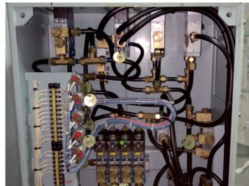
No. 84 86 88 90 in Valve Box
