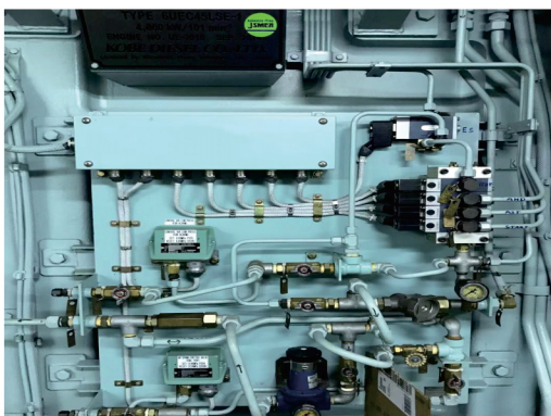
UEC Refit after Overhaul
